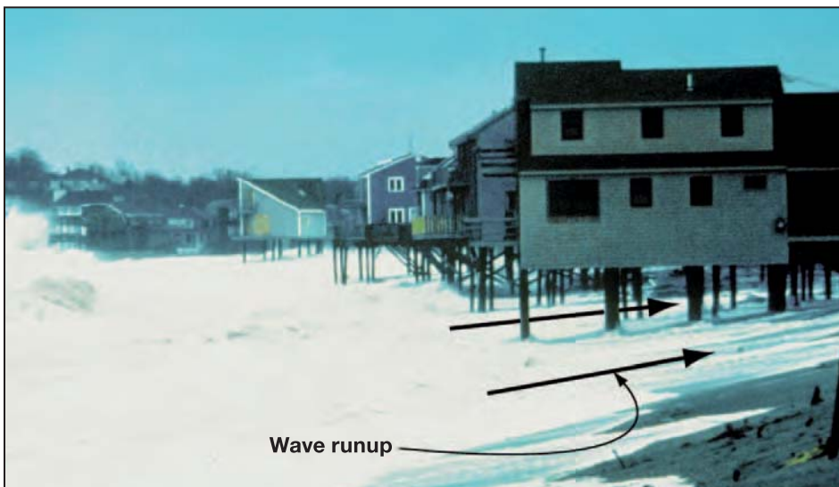
Figure 3-24. Wave runup beneath elevated buildings at Scituate, MA, during the December 1992 nor'easter storm SOURCE: JIM O'CONNELL, USED WITH PERMISSION
