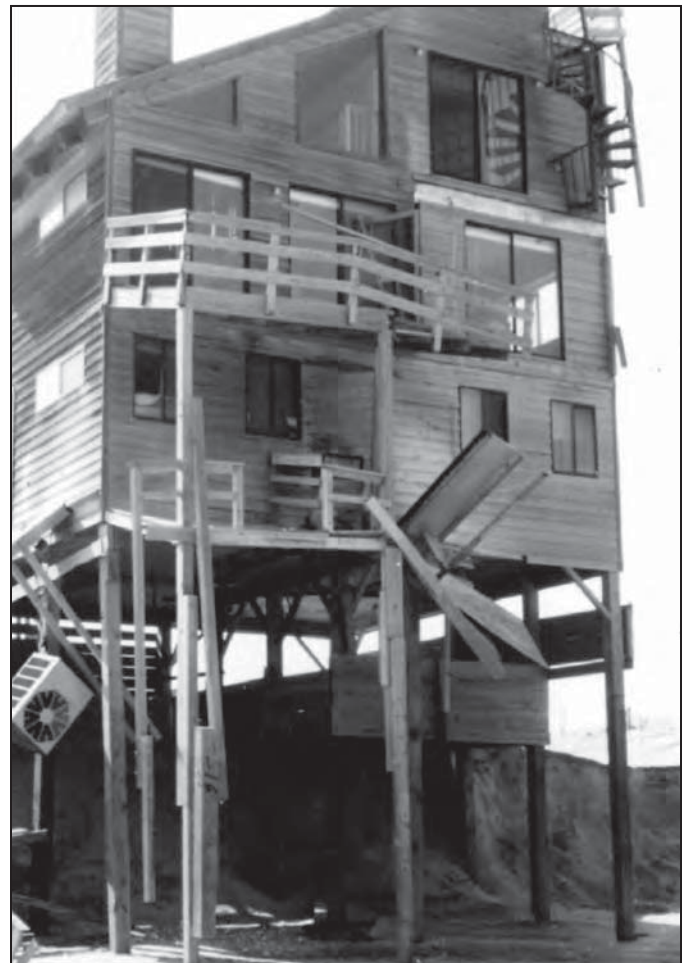
Figure 2-3. Although this house seems to have lost only several decks and a porch during the March 1989 nor'easter, the loss of supporting soil due to long-term erosion left its structural integrity in question following successive storms
